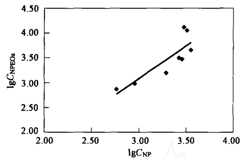
Fig. 3 Relationship between the concentration of NP and NPEOs in the sedimentary core from Beipaiming Channel, China ( p < 0.001 , r^2 = 0.7387 ).
