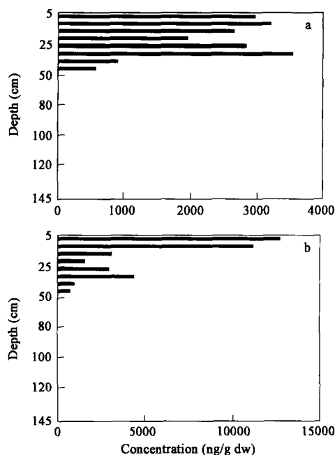
Fig. 2 Concentration profiles of NP(a) and NPEOs(b) in sedimentary core from Beipaiming Channel.
