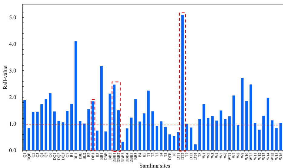
Figure 3. Ratio ( R_{\text{all}} -value) of SAs and their metabolites in STP effluent, wastewater from discharge sites, and river water samples in Wenyu River Basin. Dotted boxes indicate discharge sites with R_{\text{all}} -values greater than 1.1.
