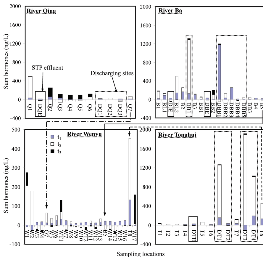
FIGURE 4. PCA-MLR source contribution plots for all water samples including river, discharged, and STP composite effluent samples. Sampling sites are shown in FIGURE 1. t_1 : treated sewage and/or naturally attenuated untreated sewage. t_2 : freshly discharged untreated sewage. t_3 : a different source from domestic sewage.
